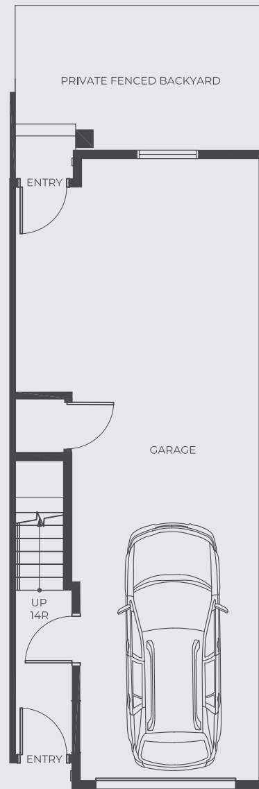
GARAGE
