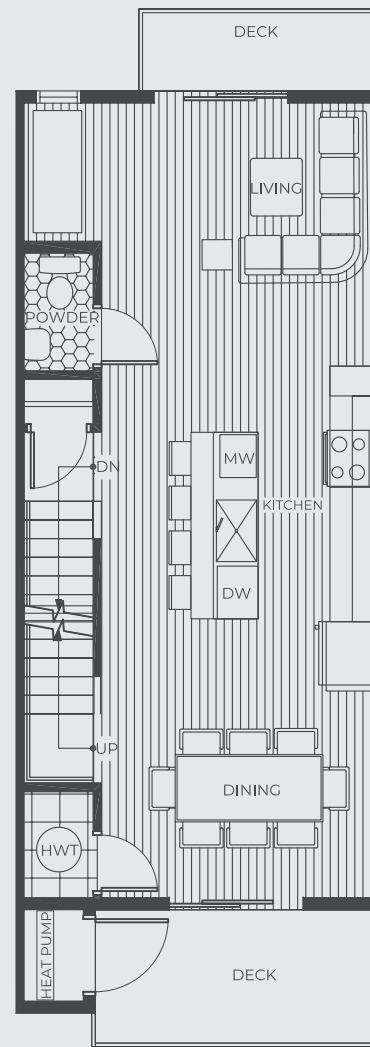
MAIN FLOOR
