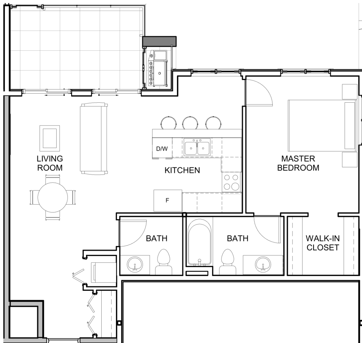
Floor 1
