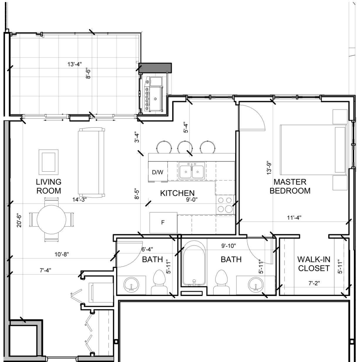
Floor 1
