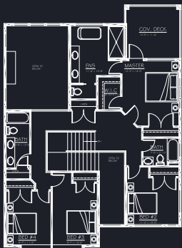
UPPER FLOOR
